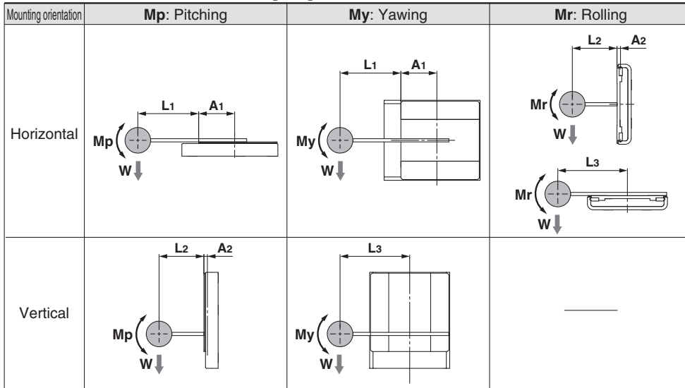
Fig. 2 Allowable Load Mass: W_{max} [g]
