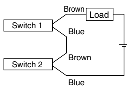
2-wire with 2-switch AND connection
