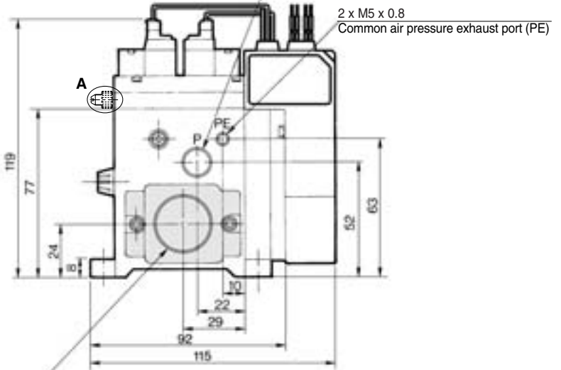
1/2, 3/4 (Rc, NPTF, G) Common exhaust port (EXH)
